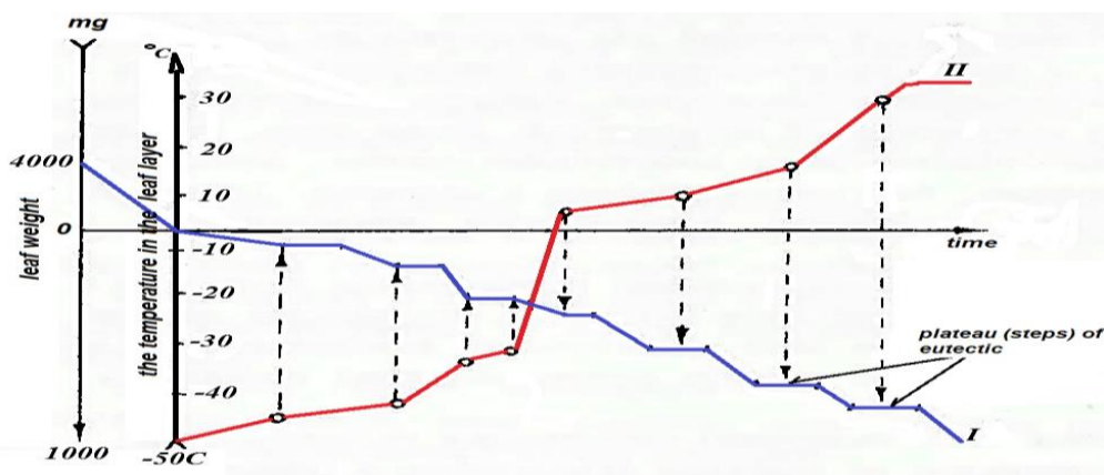
Fig. 1 Averaged drying curves and temperature curves of mulberry leaf with emerging eutectic plates
