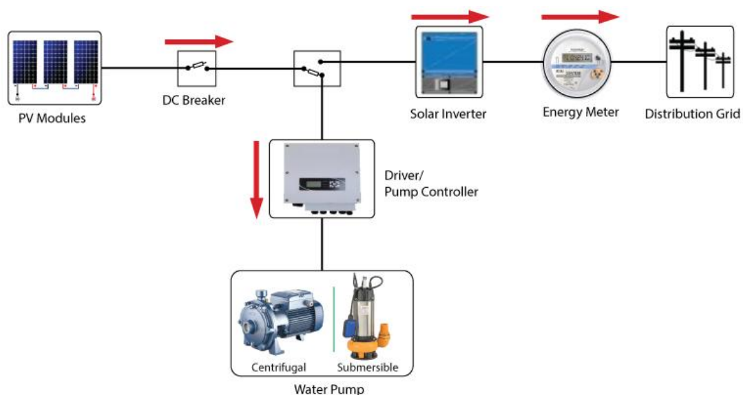
Fig. 1. Connection diagram according to the SIP grid integration guidelines
