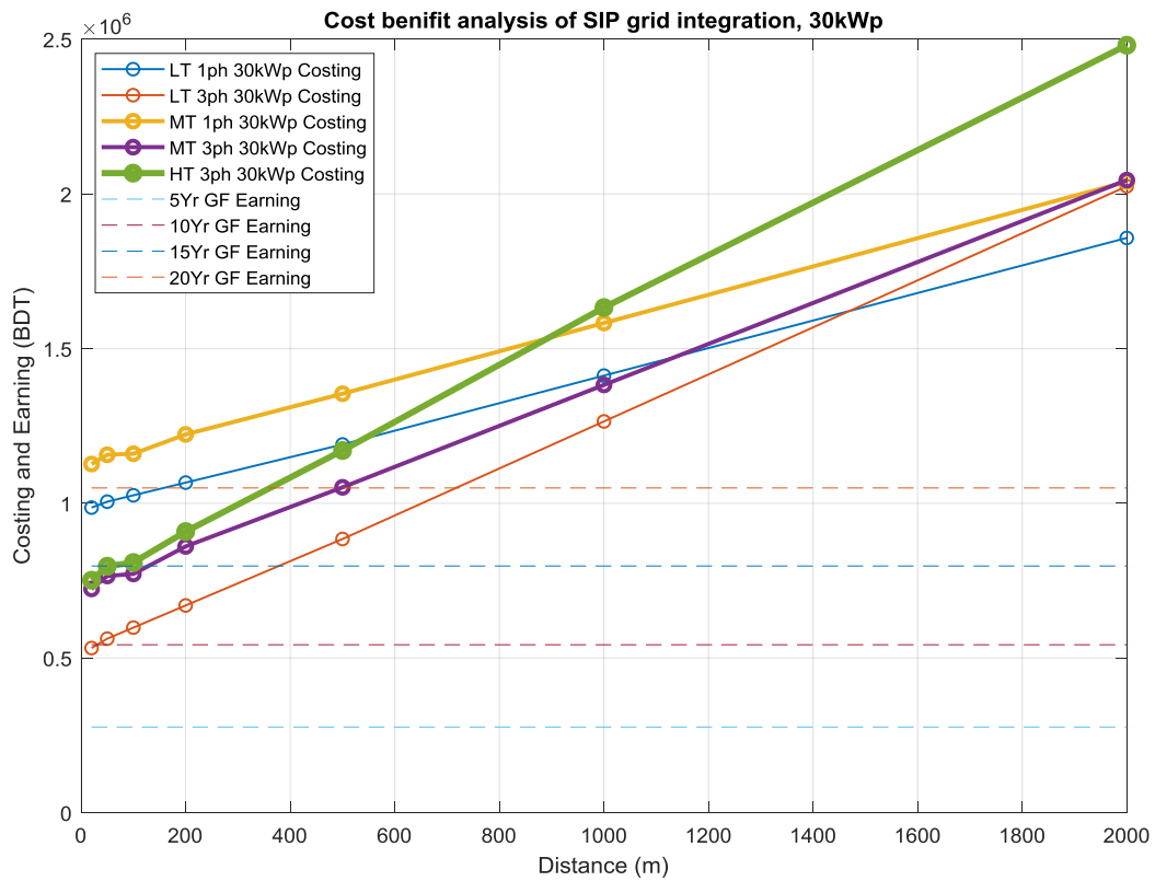
Fig. 9. Cost-benefit analysis of a 30 kWp SIP grid integration
