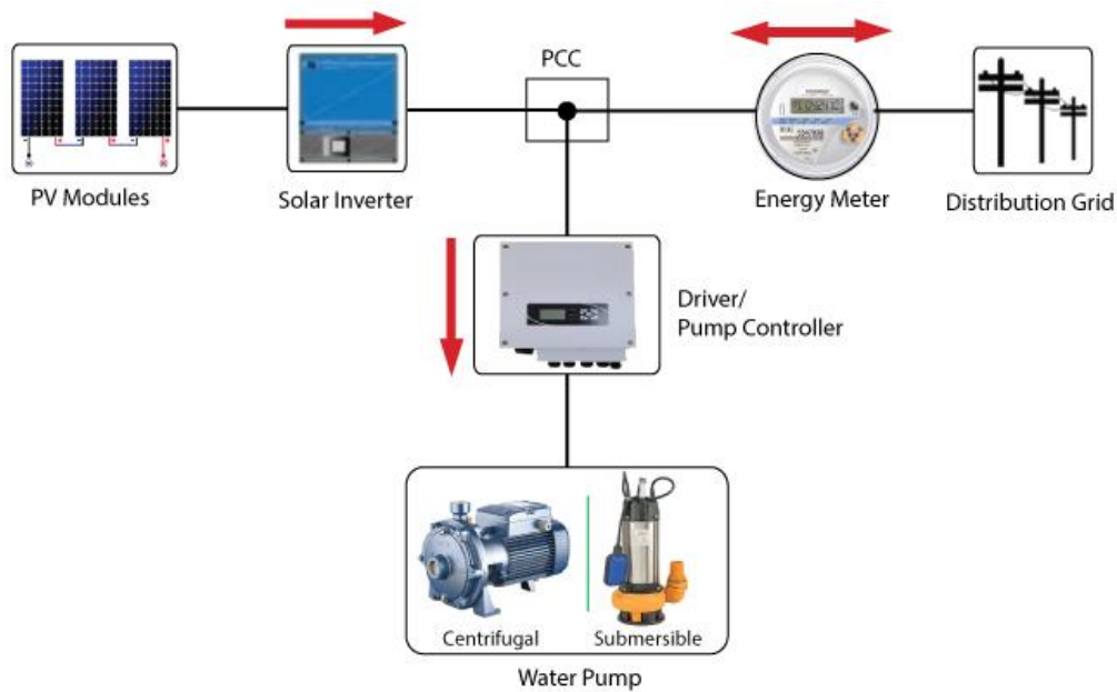
Fig. 2. Connection diagram according to the Net Metering Guidelines
