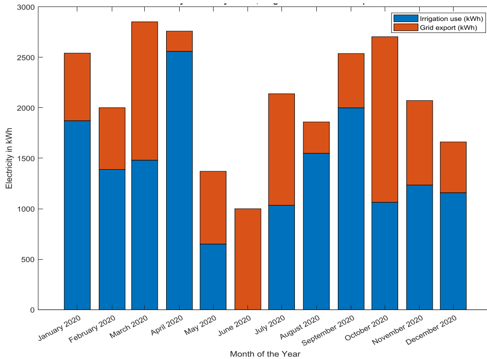
Fig. 6. Comparative energy review for irrigation use vs grid export
