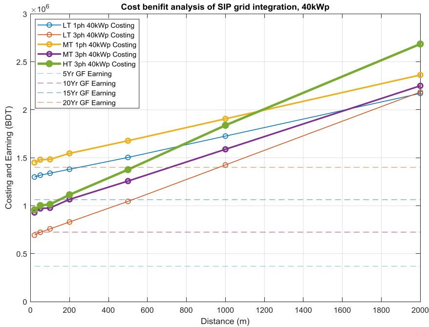
Fig. 10. Cost-benefit analysis of a 40 kWp SIP grid integration
