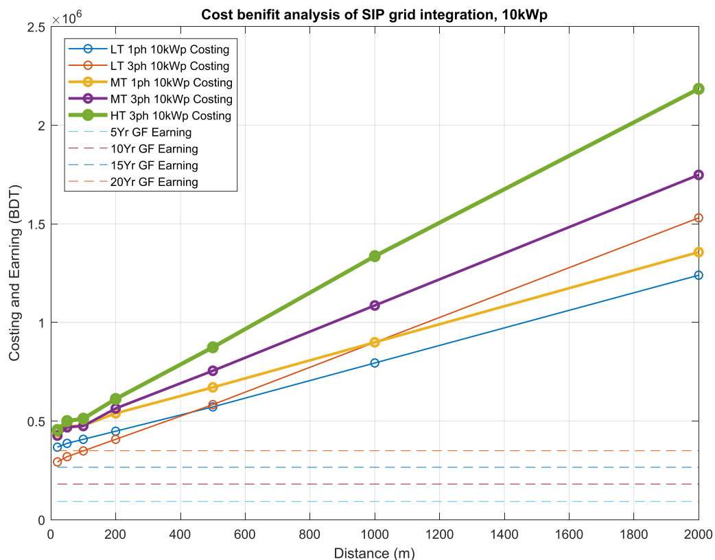
Fig. 7. Cost-benefit analysis of a 10kWp SIP grid integration
