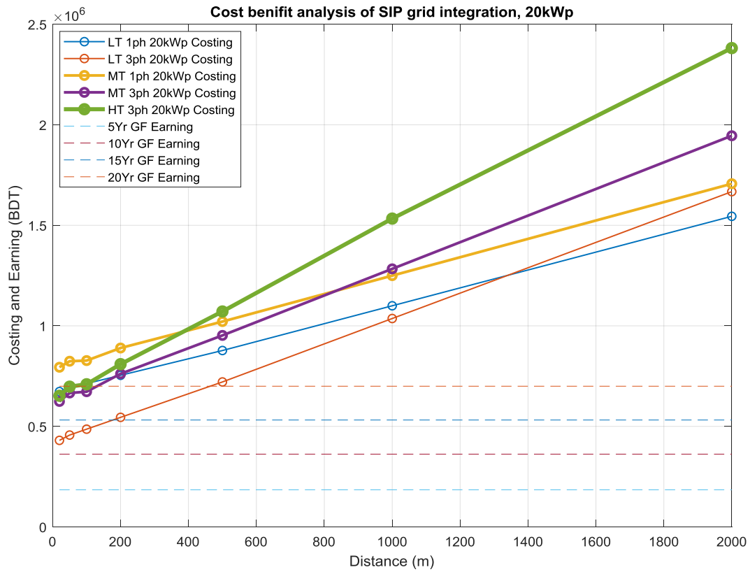
Fig. 8. Cost-benefit analysis of a 20 kWp SIP grid integration
