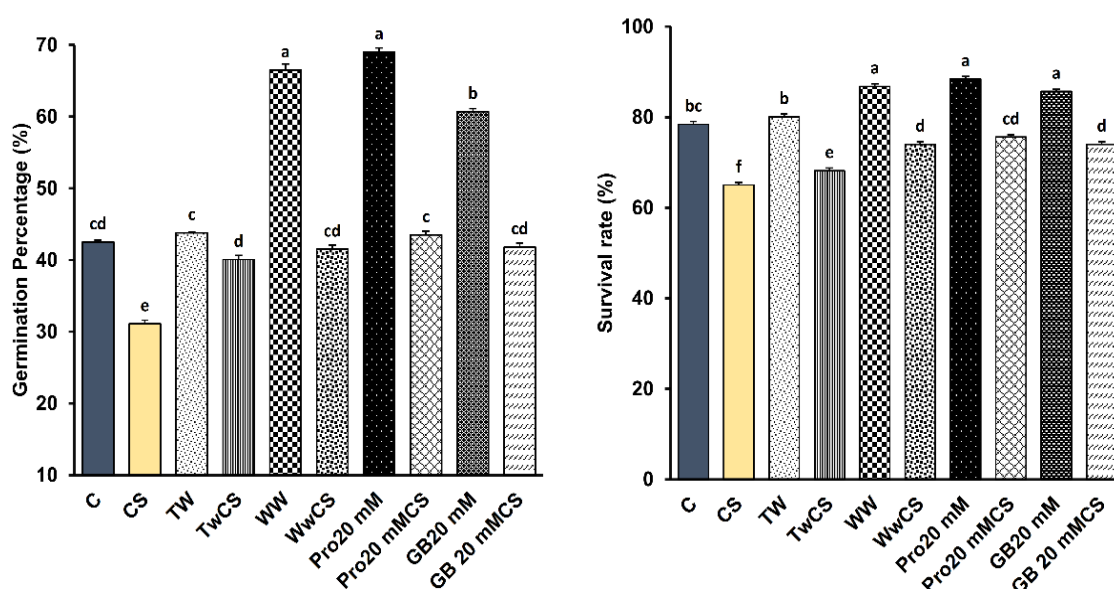
Fig. 1. Effects of different priming agents on germination percentage and survival rate of rice under chilling stress
