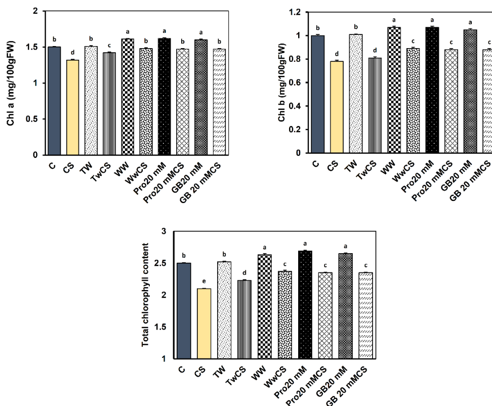
Fig. 2. Effects of different priming agents on photosynthetic pigments of rice under chilling stress
