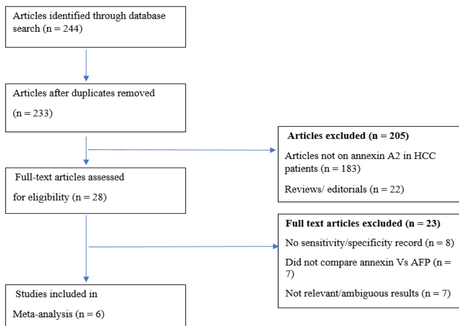
Fig. 1. Study selection map showing the literature search, evaluation, inclusion and exclusion
