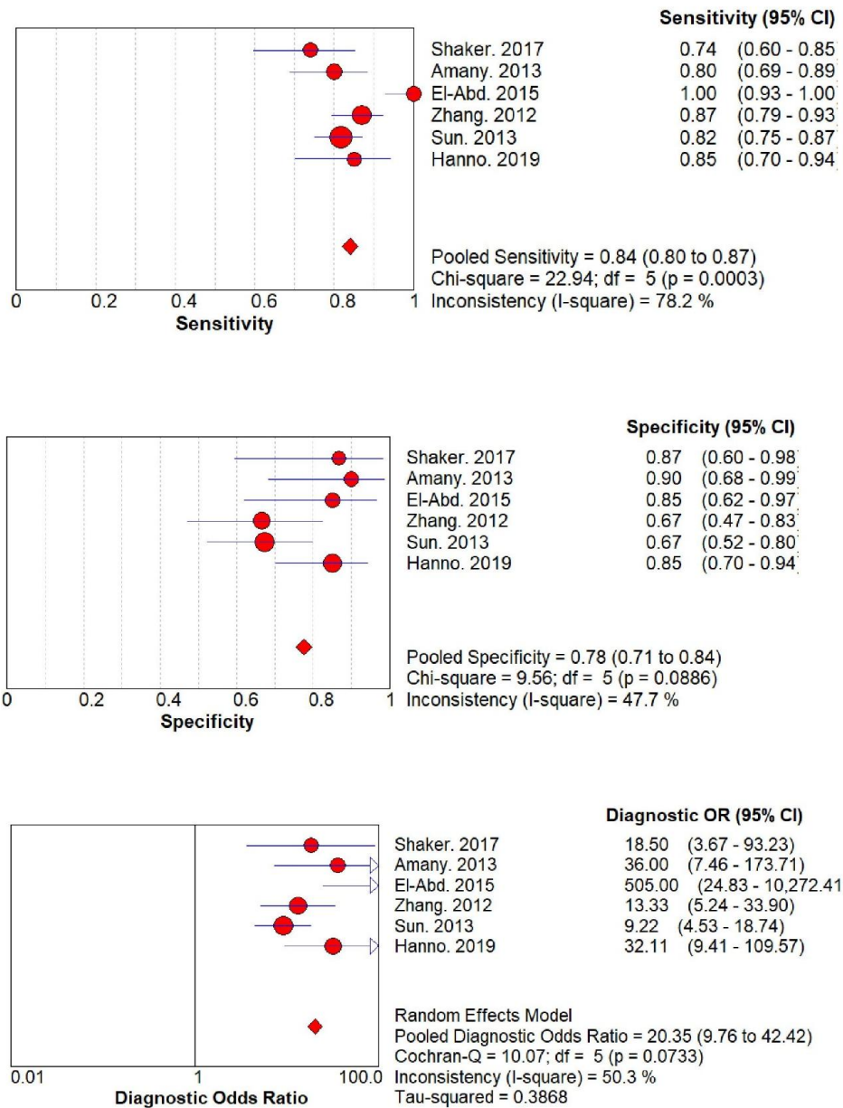
Fig. 2. Sensitivity, specificity and diagnostic odds ratio of annexin A2 in HCC
