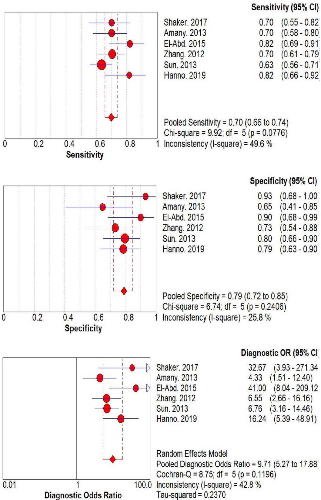
Fig. 3. Sensitivity, specificity and diagnostic odds ratio of AFP in HCC
