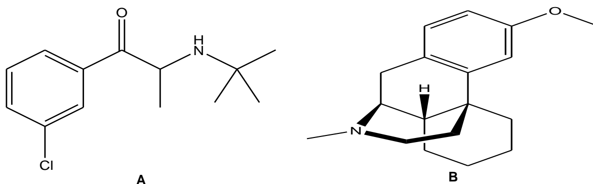
Fig. 1. Chemical structures of (A) Bupropion and (B) Dextromethorphan
