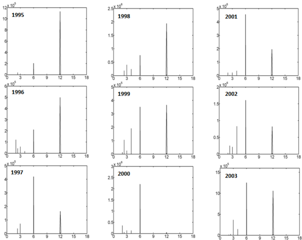
Fig. 4. Periodogram of electron density during daytime over 0° magnetic
