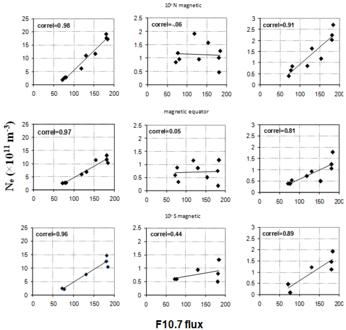
Fig. 9. Amplitude of mean, annual and semiannual components of Ne (from left to right) plotted against 10.7 cm solar flux at three latitudes for day time (10:00-14:00 LT)
