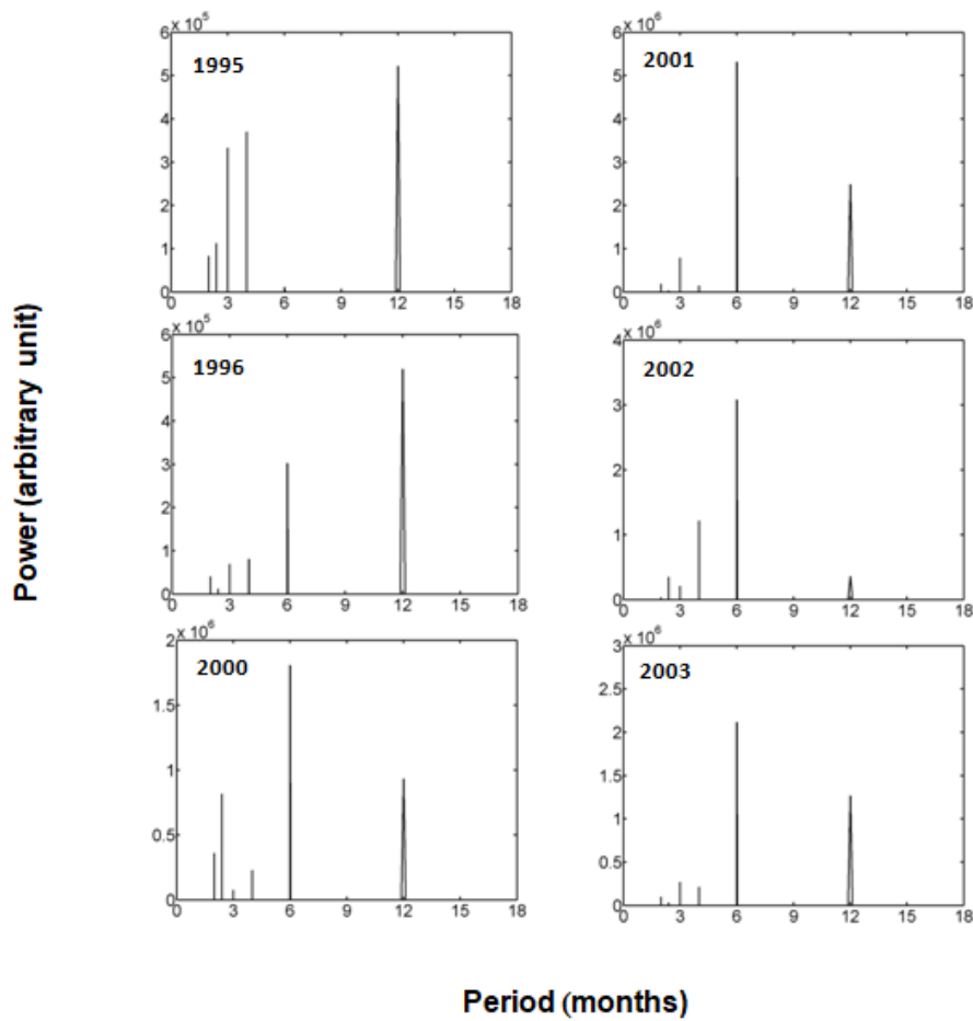
Fig. 5. Periodogram of electron density during daytime over 10° S magnetic
