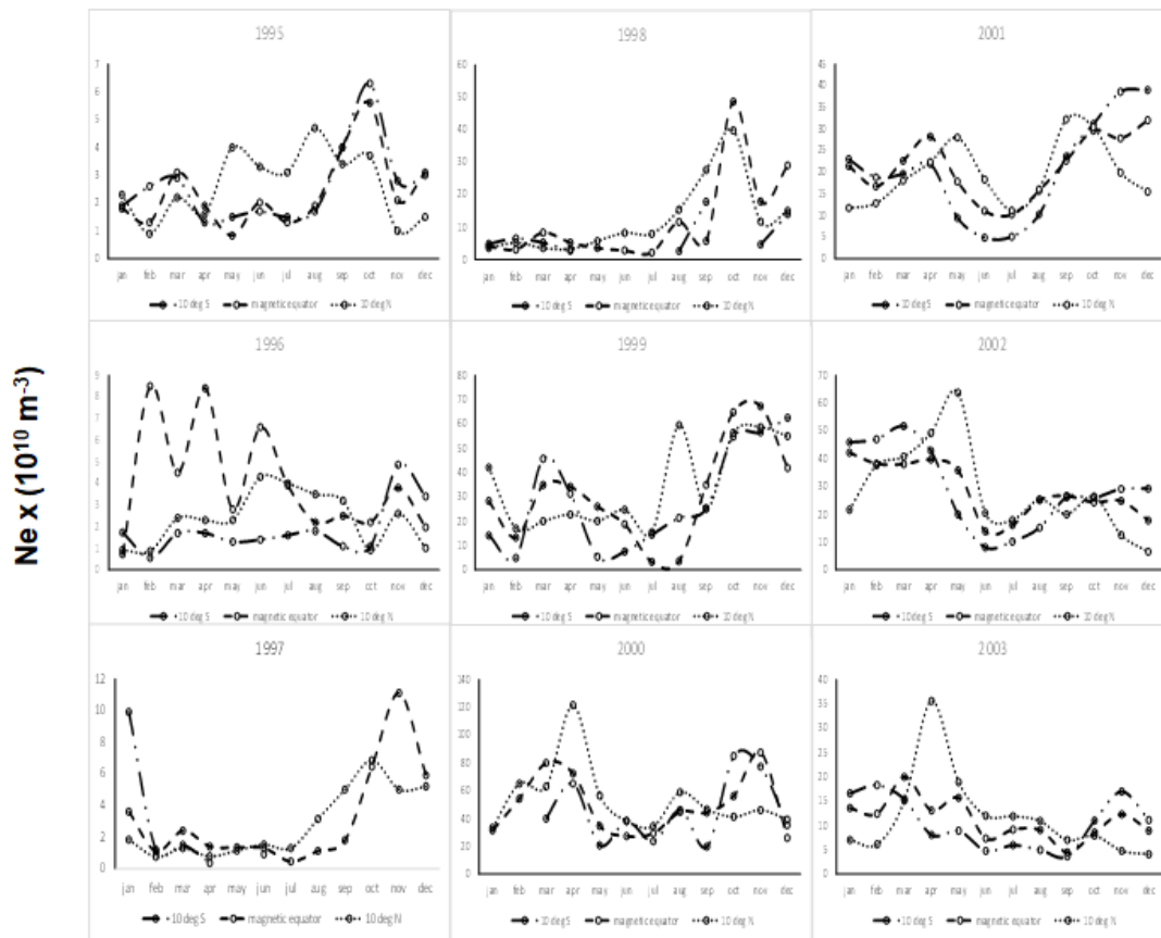
Fig. 2. Yearly variation of electron density during nighttime at 500 km altitude
