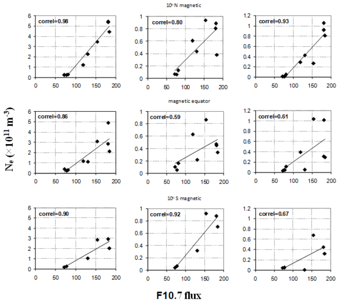
Fig. 10. Amplitude of mean, annual and semiannual components of Ne (from left to right) plotted against 10.7 cm solar flux at three latitudes for night time (22:00-00:00 LT)
