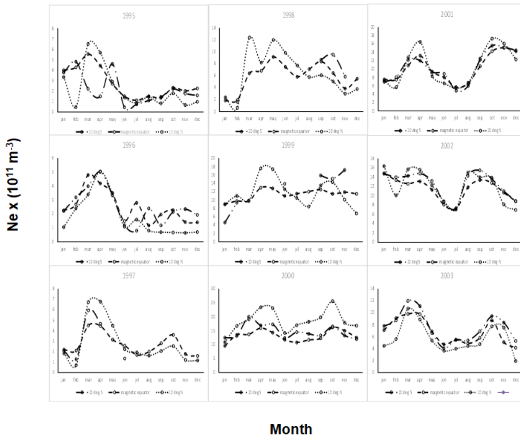
Fig. 1. Yearly variation of electron density during daytime at 500 km altitude
