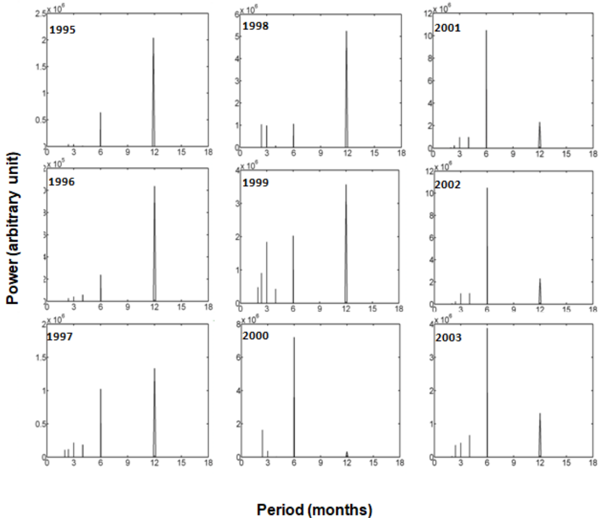
Fig. 3. Periodogram of electron density during daytime over 10° N magnetic
