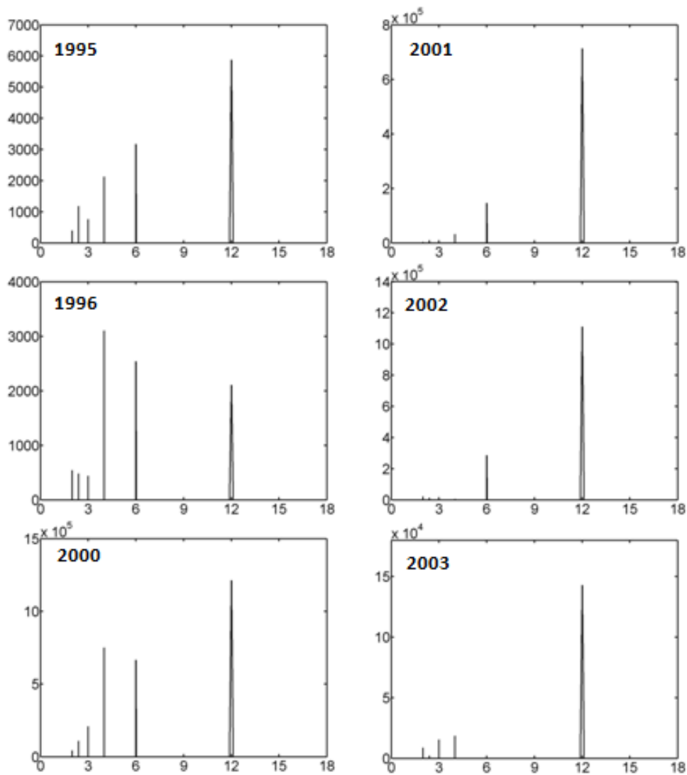
Fig. 8. Periodogram of electron density during nighttime over 10^\circ S magnetic
