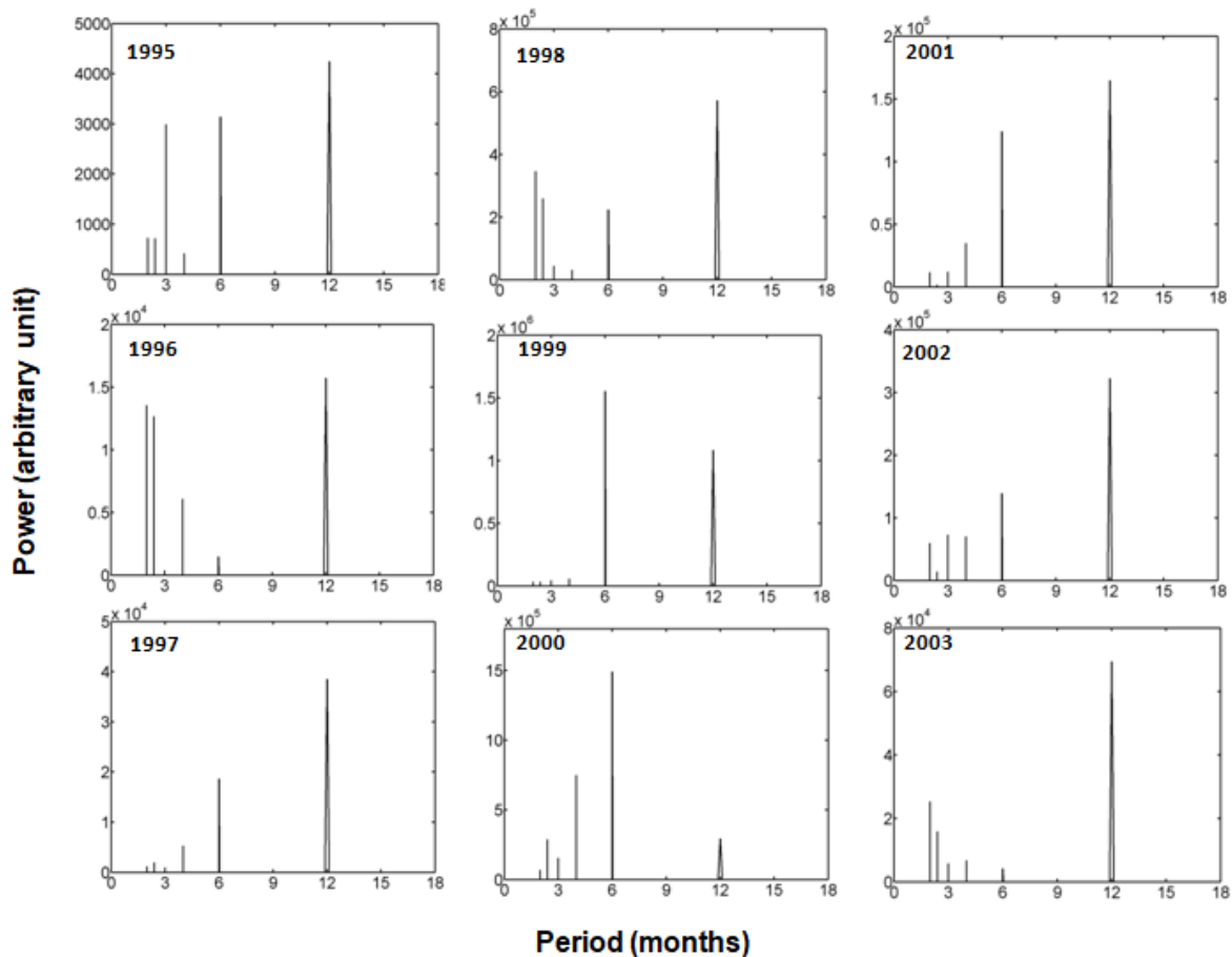
Fig. 7. Periodogram of electron density during nighttime over 0° magnetic
