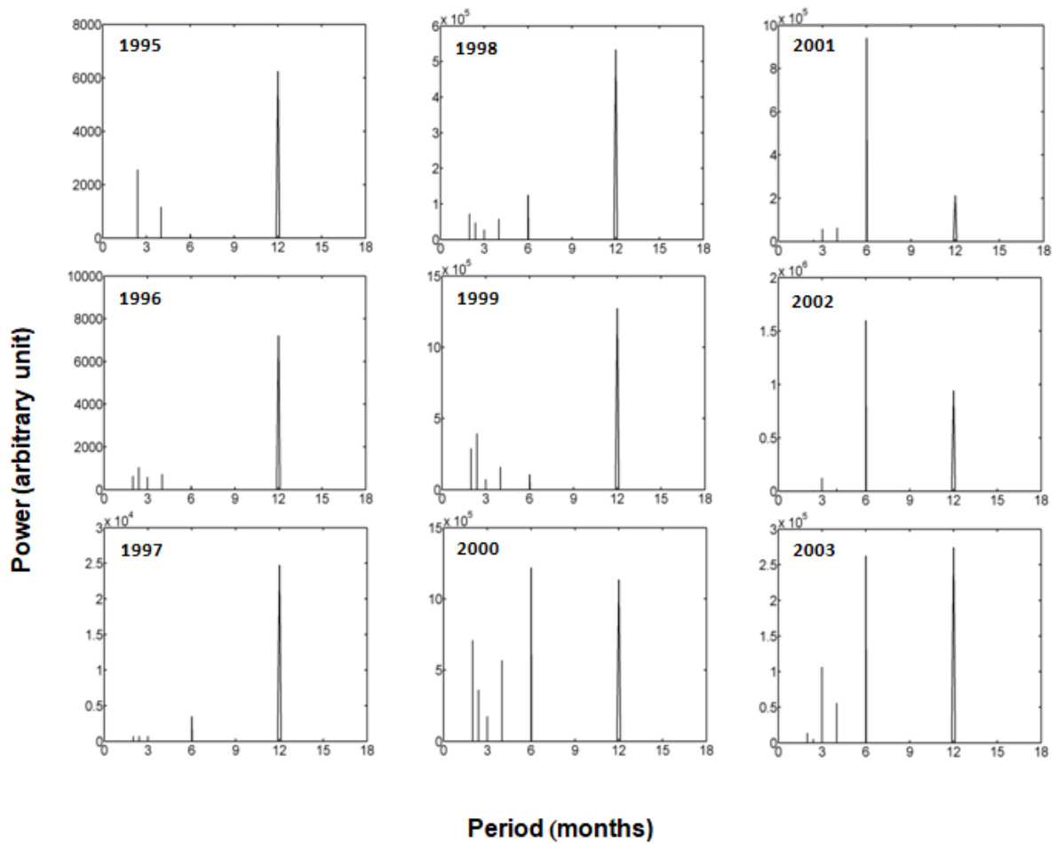
Fig. 6. Periodogram of electron density during nighttime over 10° N magnetic
