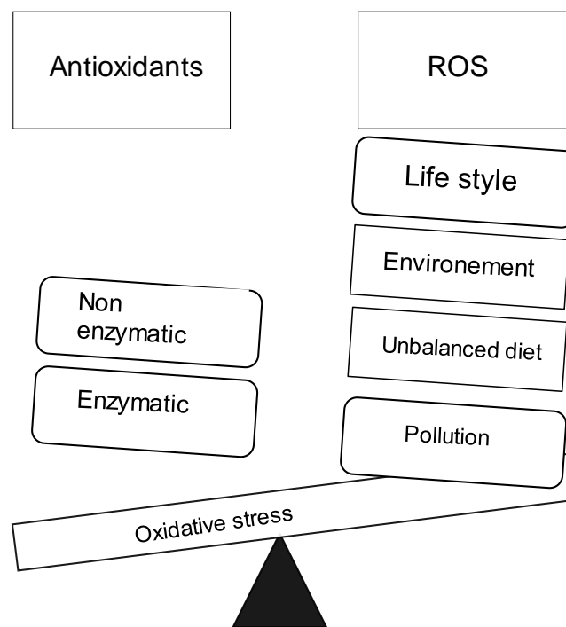
Fig. 3. Oxidative stress
