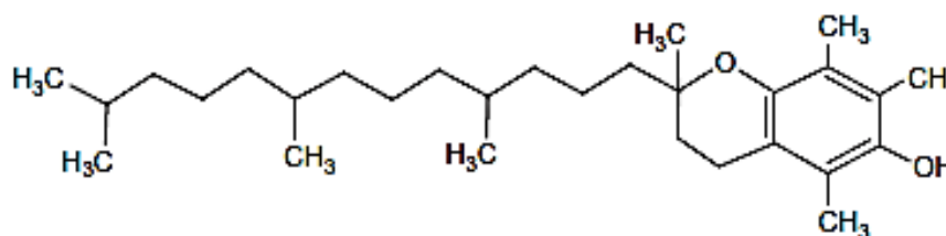
Fig. 6. Structure of \alpha -tocopherol
