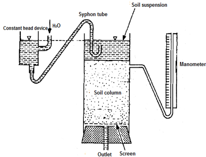
Fig. 2. A schematic diagram of the apparatus used to test the theory
