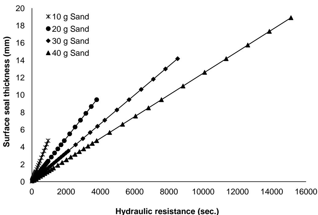
Fig. 3. Relationship between surface seal thickness and hydraulic resistance of sand particles
