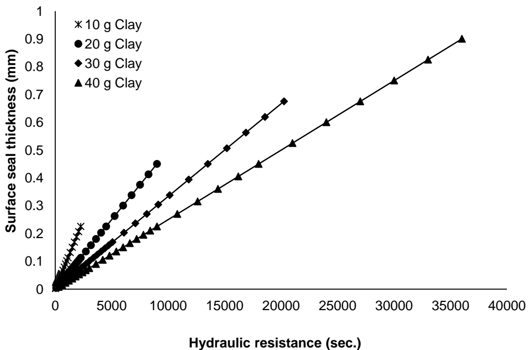
Fig. 5. Relationship between surface seal thickness and hydraulic resistance of clay particles
