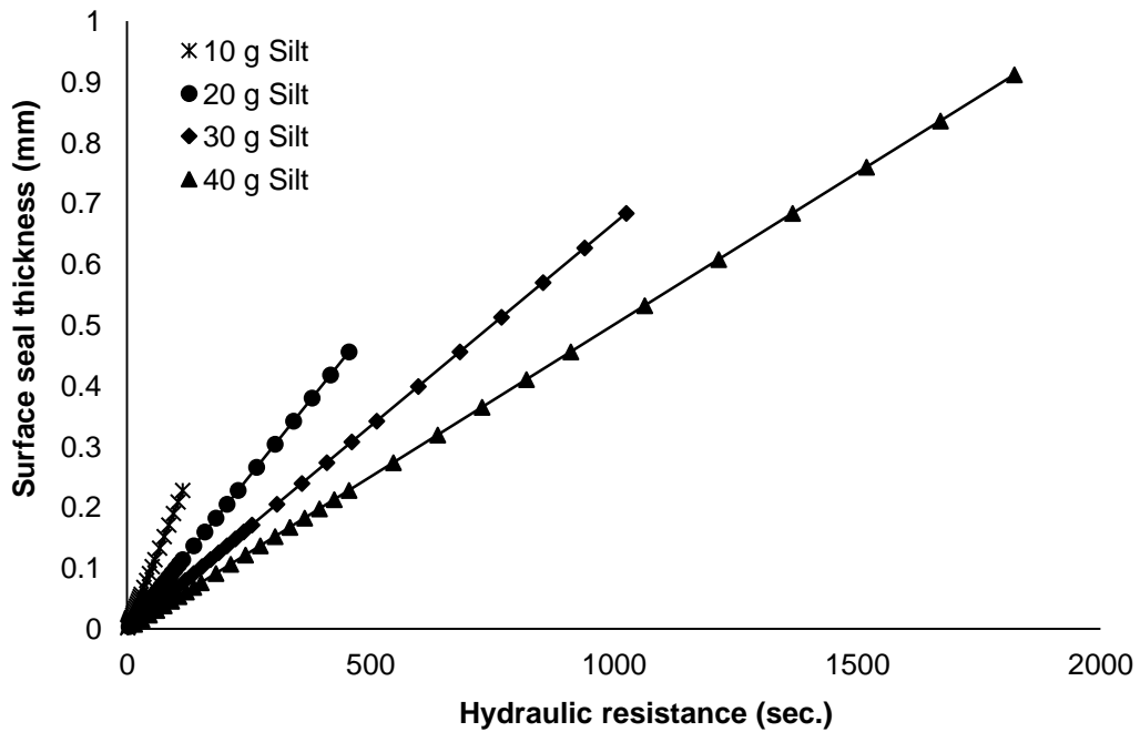
Fig. 4. Relationship between surface seal thickness and hydraulic resistance of silt particles
