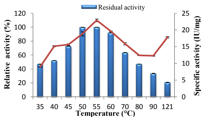
Fig. 6. Effect of temperature on purified \alpha -amylase of B. sonorensis GV2
