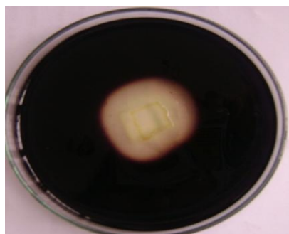
Fig. 4. Zymogram analysis of purified \alpha -amylase of B. sonorensis GV2 on starch agar plates with gel cut from Native PAGE showing zone of hydrolysis
