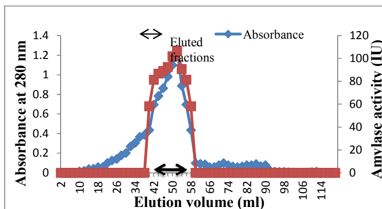
Fig. 1. Protein and enzyme activity profile of fractions of Sephadex G-75 column chromatography of the dialyzed α-amylase of B. sonorensis GV2
