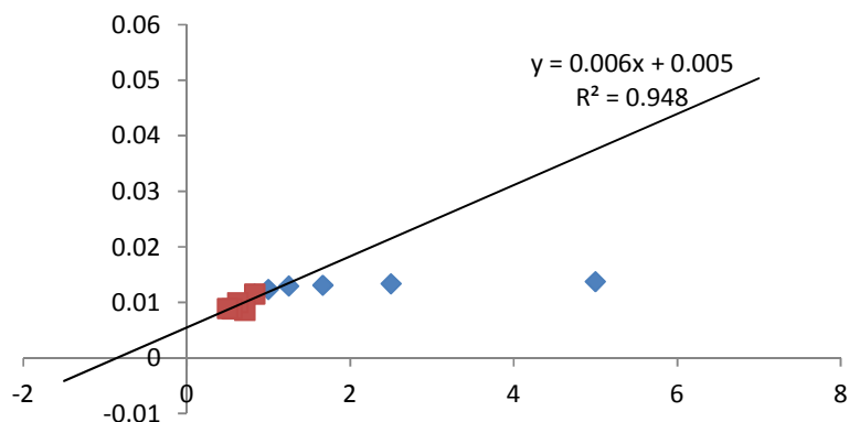
Fig. 10. Lineweaver burk plot for enzyme kinetics of B. sonorensis GV2
