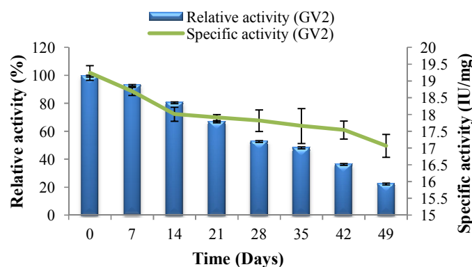
Fig. 9. Shelf stability of purified \alpha -amylase at room temperature
