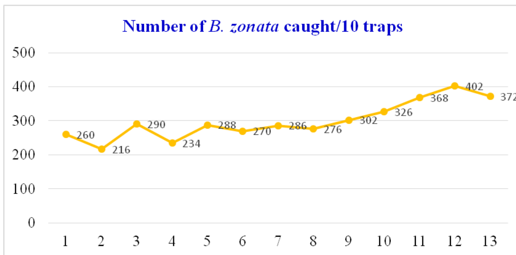
Fig. 2. Population of B. zonata from 1 st to 13 th SMW in mango orchard
