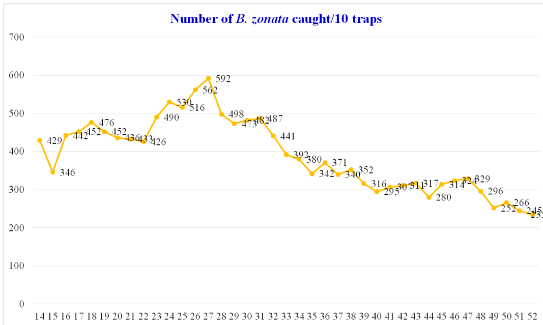
Fig. 1. Population of B. zonata from 14 th to 52 nd SMW in mango orchard
