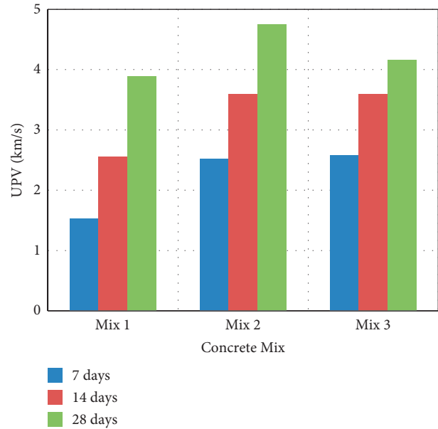
FIGURE 2: UPV value for GPC for different proportions.
