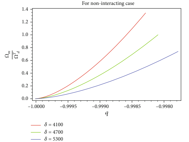
FIGURE 14: Behavior of coincidence parameter \tilde{r} = \Omega_m/\Omega_d^T against q .
